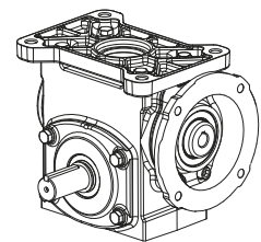
Ceiling Mounted, Motor Adapter or Input Shaft above Output Shaft
