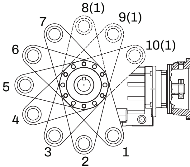
Standard Torque-Arm (KT) Possible Mounting Positions
