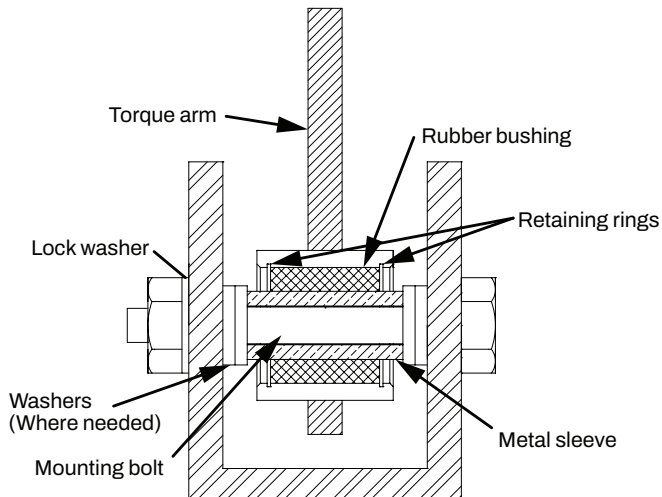
Figure 1 - Quantis Torque-Arm Mounted to Customer Bracket
