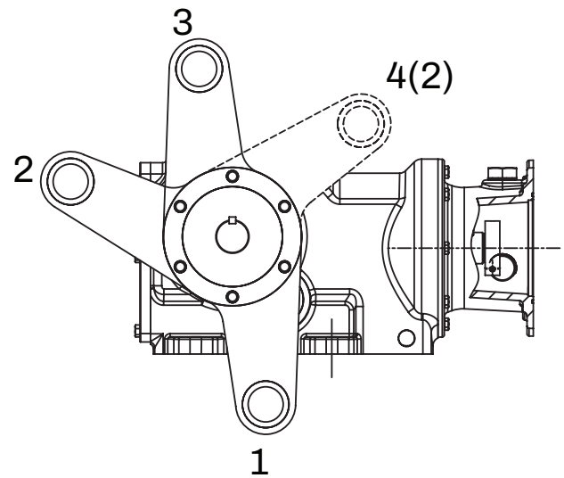
Stainless Steel Torque-Arm (KTS) Possible Mounting Positions
