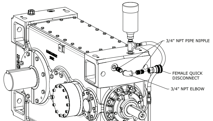
Figure 7 - Female Quick Disconnect Components Front Facing (Input Side Only)
