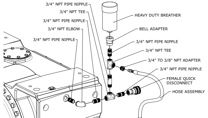
Figure 6 - Heavy Duty Breather & Female Quick Disconnect Components (Output Side Only)
