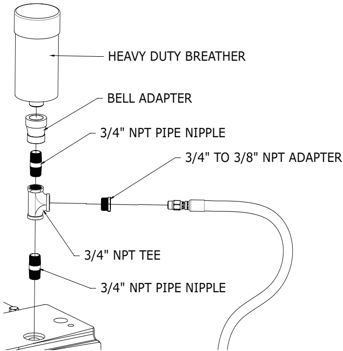
Figure 5 - Heavy Duty Breather Components
