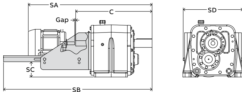
CR100 Maxum XTR scoop mount with AC motors ♦
