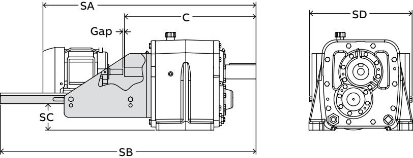
CR50 Maxum XTR scoop mount with AC motors ♦
