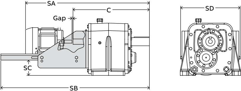
CR120 Maxum XTR scoop mount with AC motors ♦
