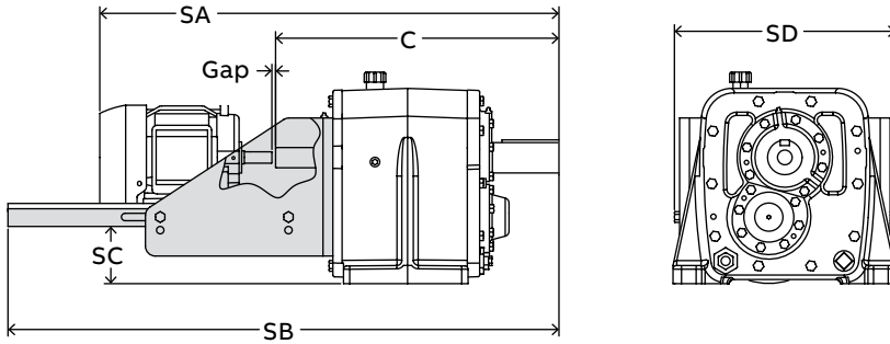
CR110 Maxum XTR scoop mount with AC motors ♦
