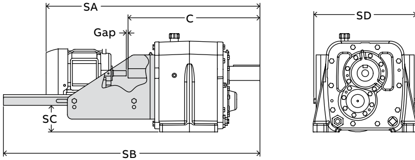
CR130 Maxum XTR scoop mount with AC motors ♦
