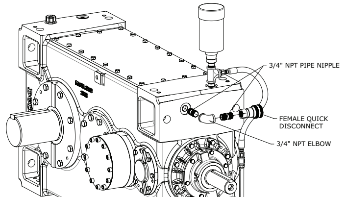
Figure 6 - Female Quick Disconnect Components Front-Facing
