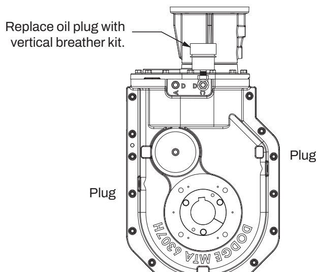
Figure 4 - Installed Position D Breather Kit Replaces Standard Breather
