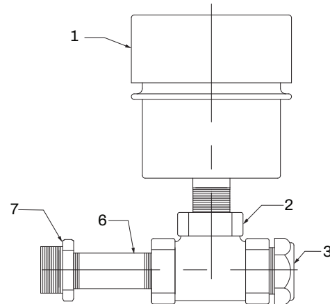
Figure 2 - Position D Breather Kit (MTA4-MTA8)
