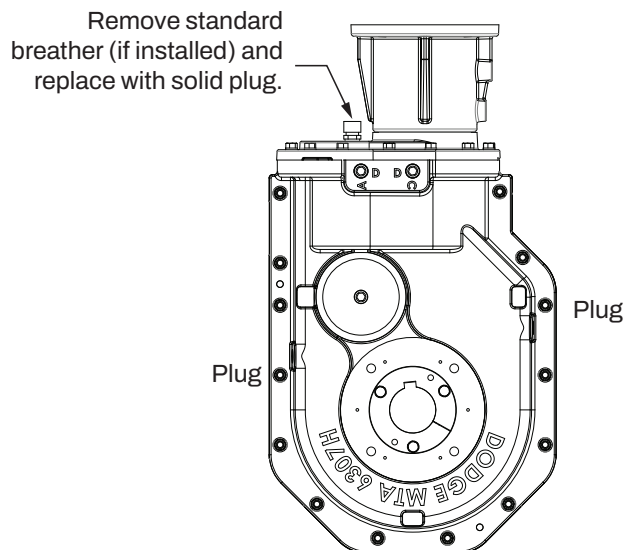
Figure 3 - Installing Position D Breather Kit Top Oil Plug Replacement
