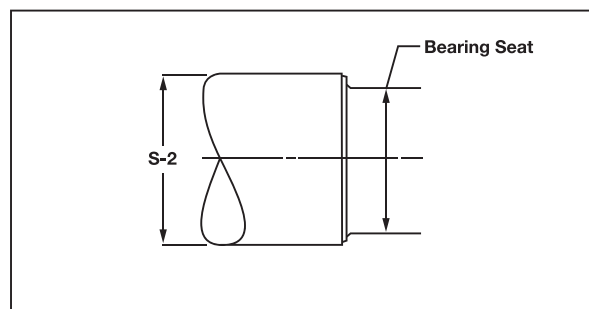
Figure 2 - Shaft Diameter
