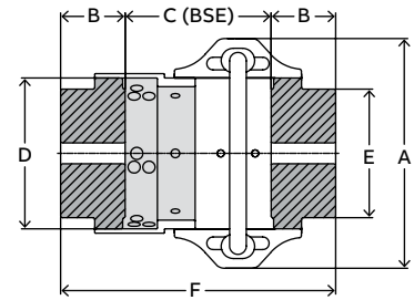
Half spacer - outboard
