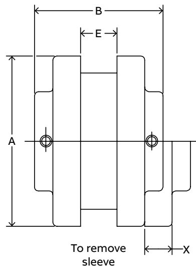
Type “S” coupling
