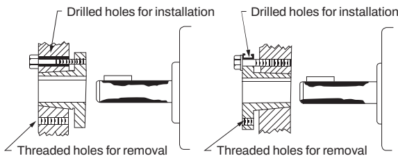
Figure 1 - Conventional Mounting
