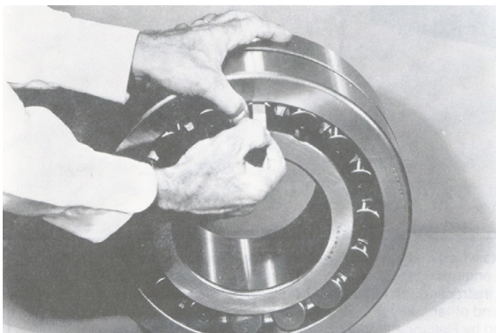
Figure 1 - Internal clearance
