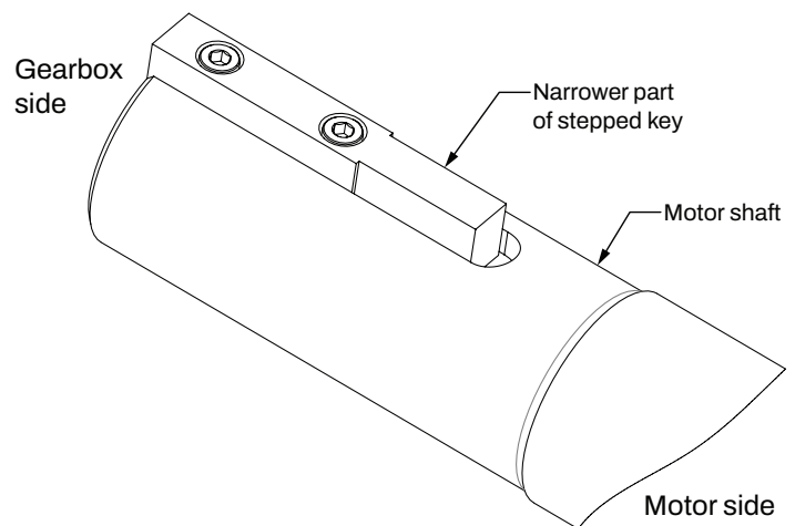
Figure 1 - Stepped key orientation when seated on motor shaft
