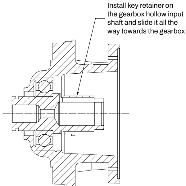
Figure 5 - Install key retainer on the gearbox hollow shaft. Avoid lining up the split in the key retainer with the keyway on the hollow shaft
