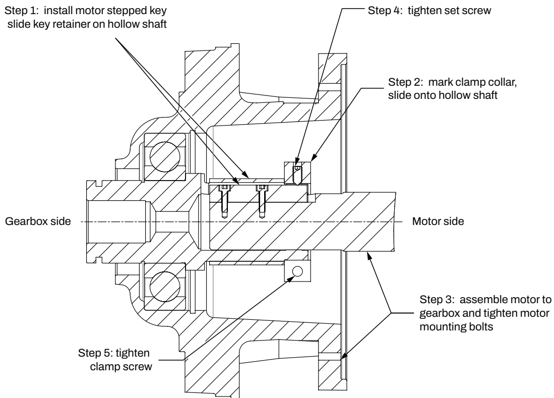
Figure 9 - Summary of installation instructions. Please review details above.
