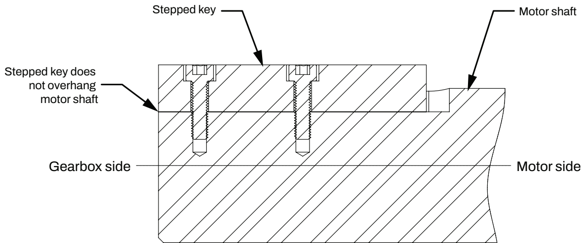
Figure 2 - CORRECT Installation method of motor stepped key if clearance holes in the key align with motor tapped holes
