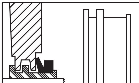
Figure 2 - Patented Triple-Test Seal
