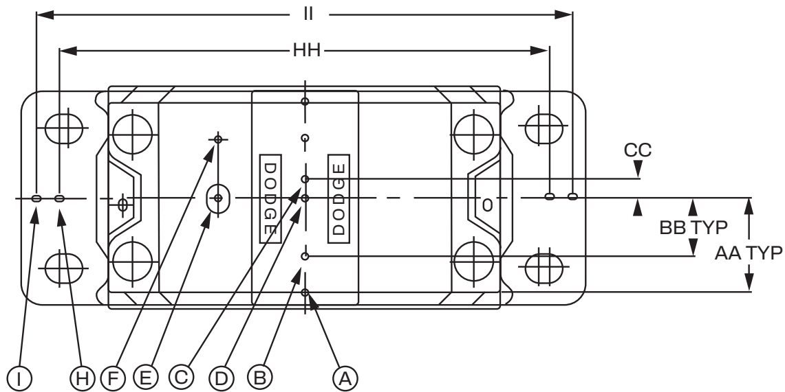
Figure 4 - USDAF Housing Dimensional and Descriptive Drawing
