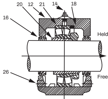
Figure 3 - Adapter Mount Parts
