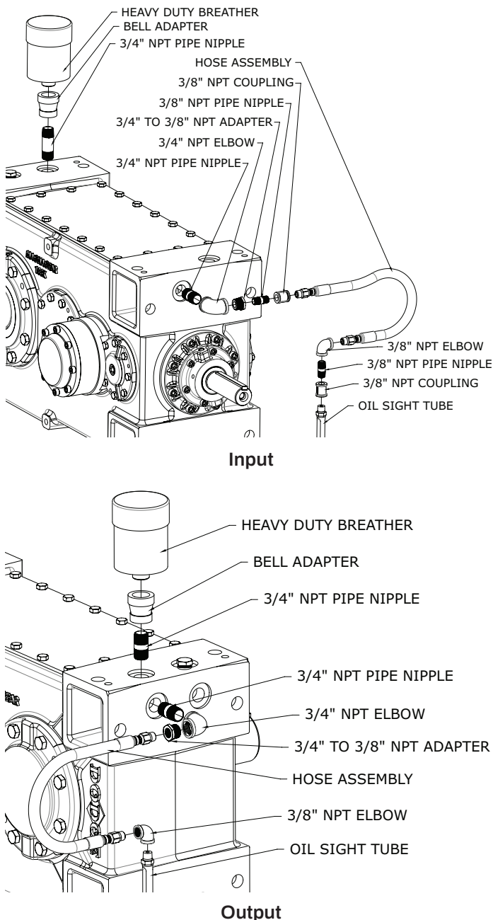
Figure 5 - Heavy Duty Breather and Oil Sight Tube Components
