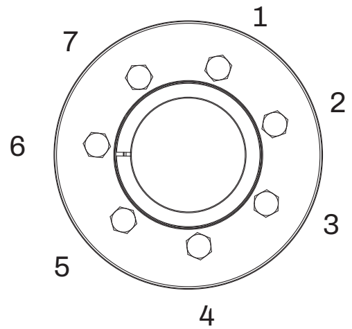
Figure 2 - Tightening Torque Pattern
