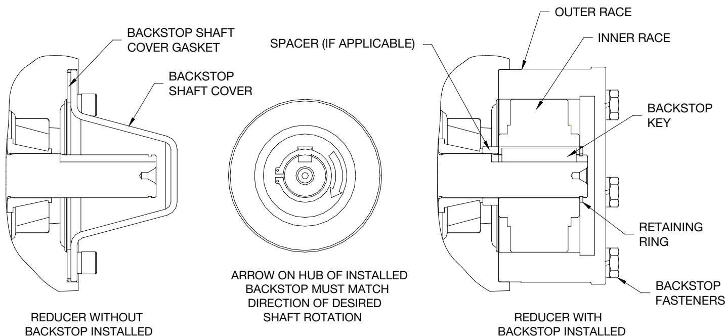
Figure 7 - Backstop Assembly
