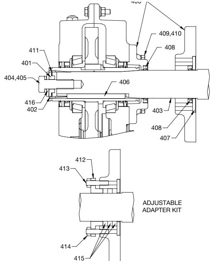
Figure 15 - Screw Conveyor Adapter Assembly
