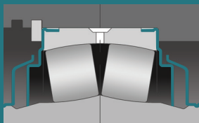
Labyrinth seal
