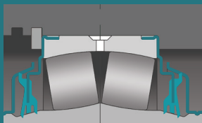
Trident seal
