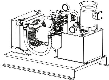
Figure 1 - Cool Lube 2
